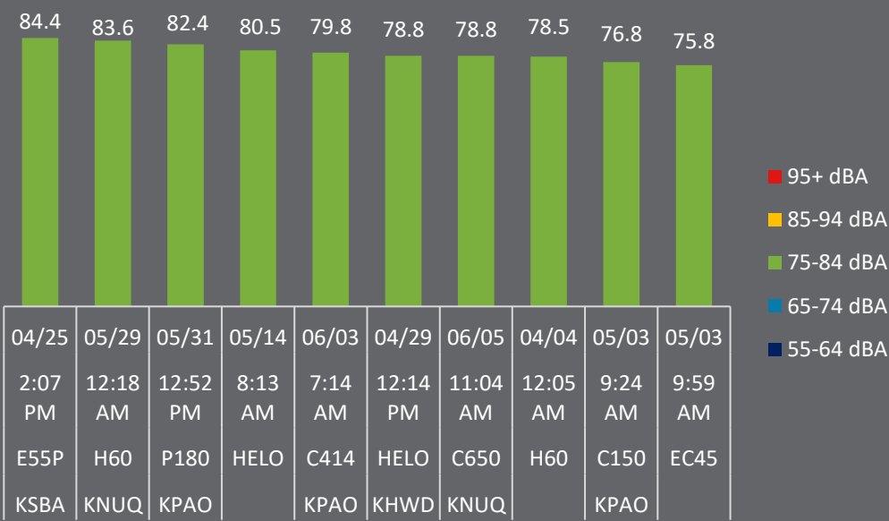
SYV-4 TOP 10 AIRCRAFT NOISE EVENTS IN Q2-2025
